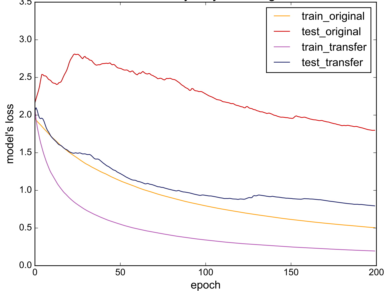
Source: WordsSynonyms - Target: FISH
