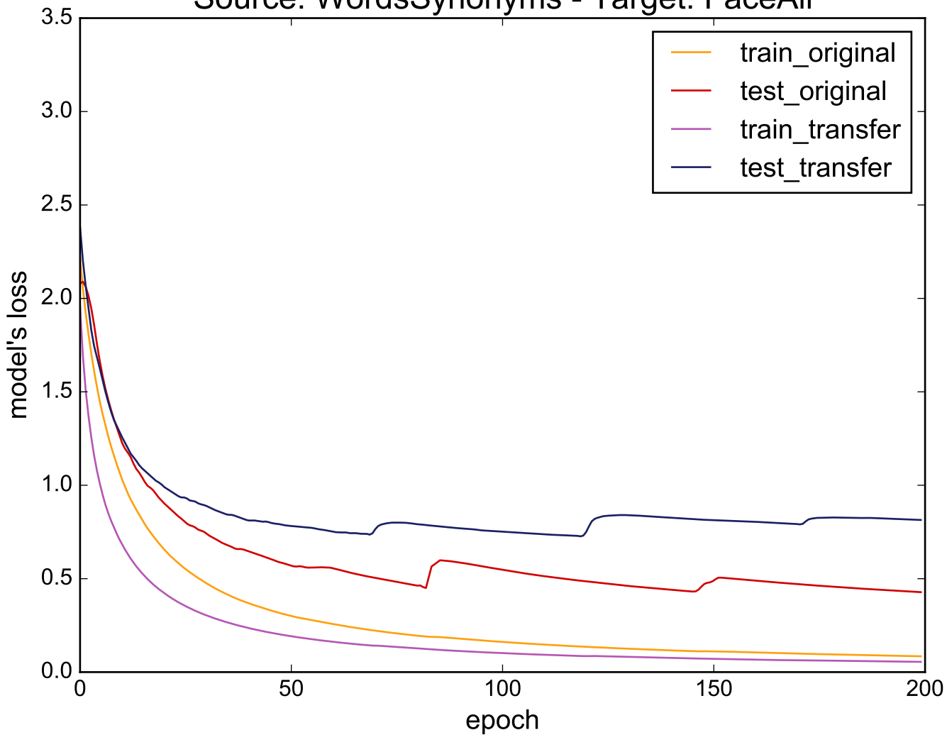
Source: WordsSynonyms - Target: FaceAll
