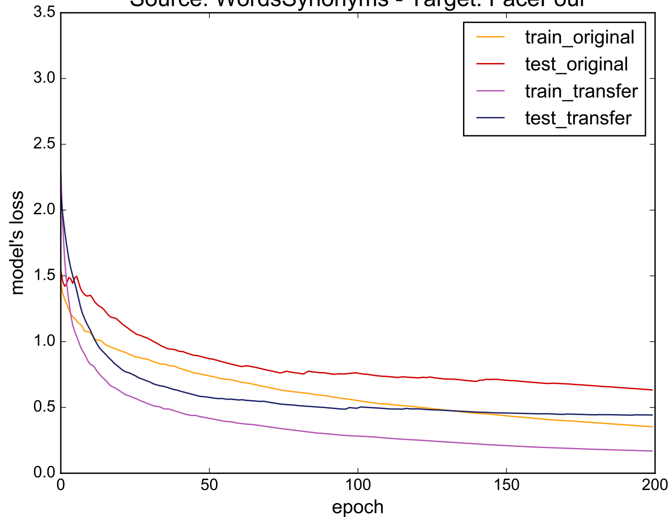
Source: WordsSynonyms - Target: FaceFour
