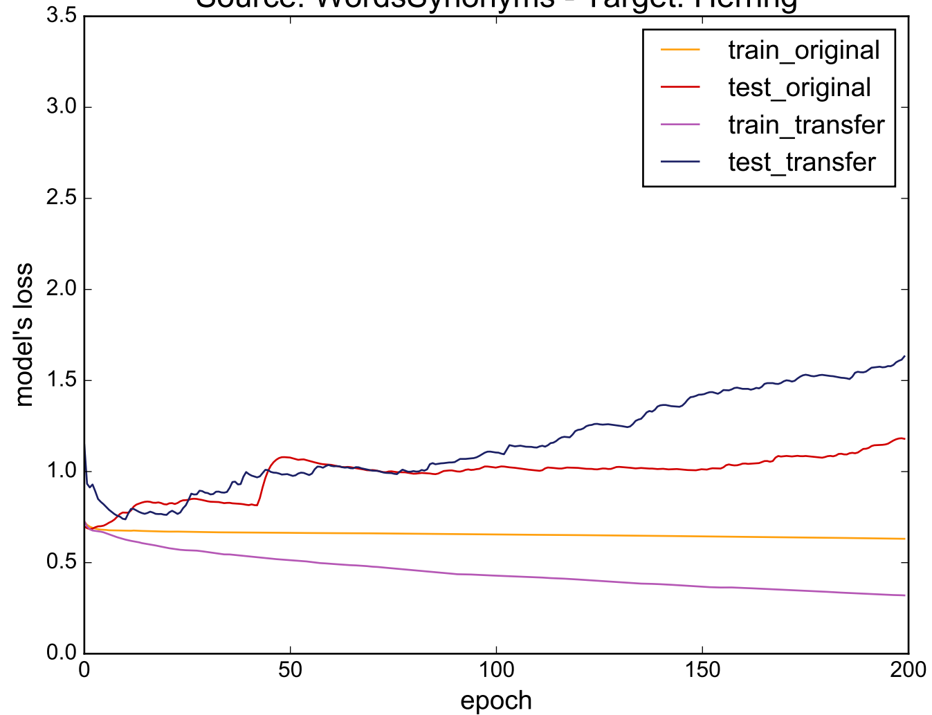
Source: WordsSynonyms - Target: Herring
