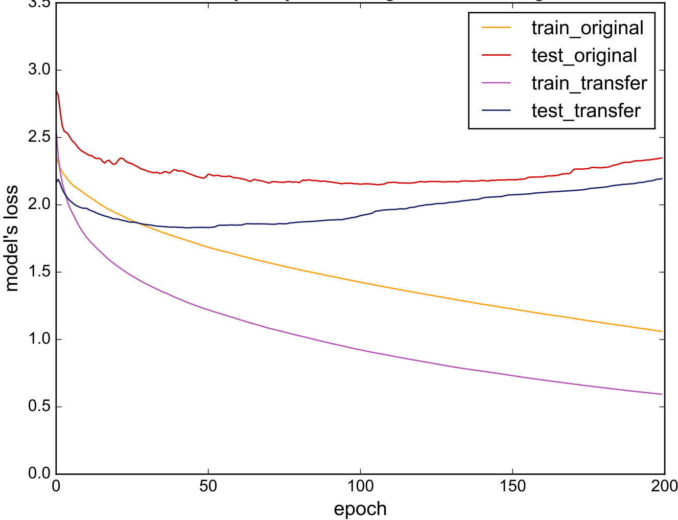
Source: WordsSynonyms - Target: InsectWingbeatSound
