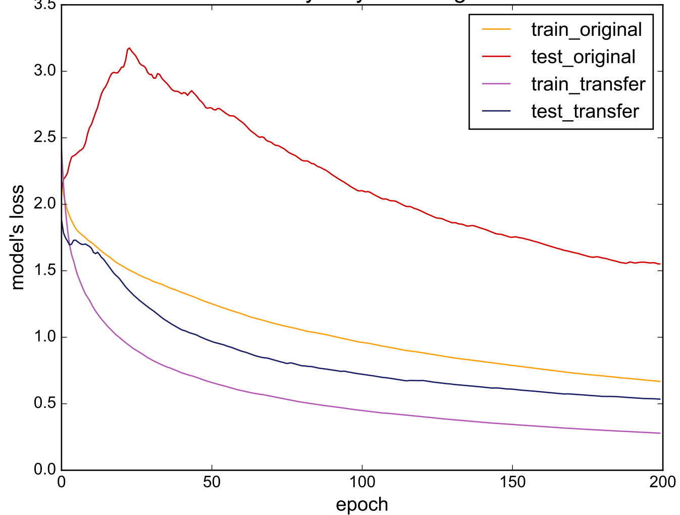
Source: WordsSynonyms - Target: MALLAT
