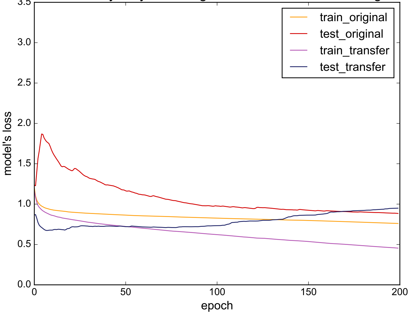
Source: WordsSynonyms - Target: MiddlePhalanxOutlineAgeGroup
