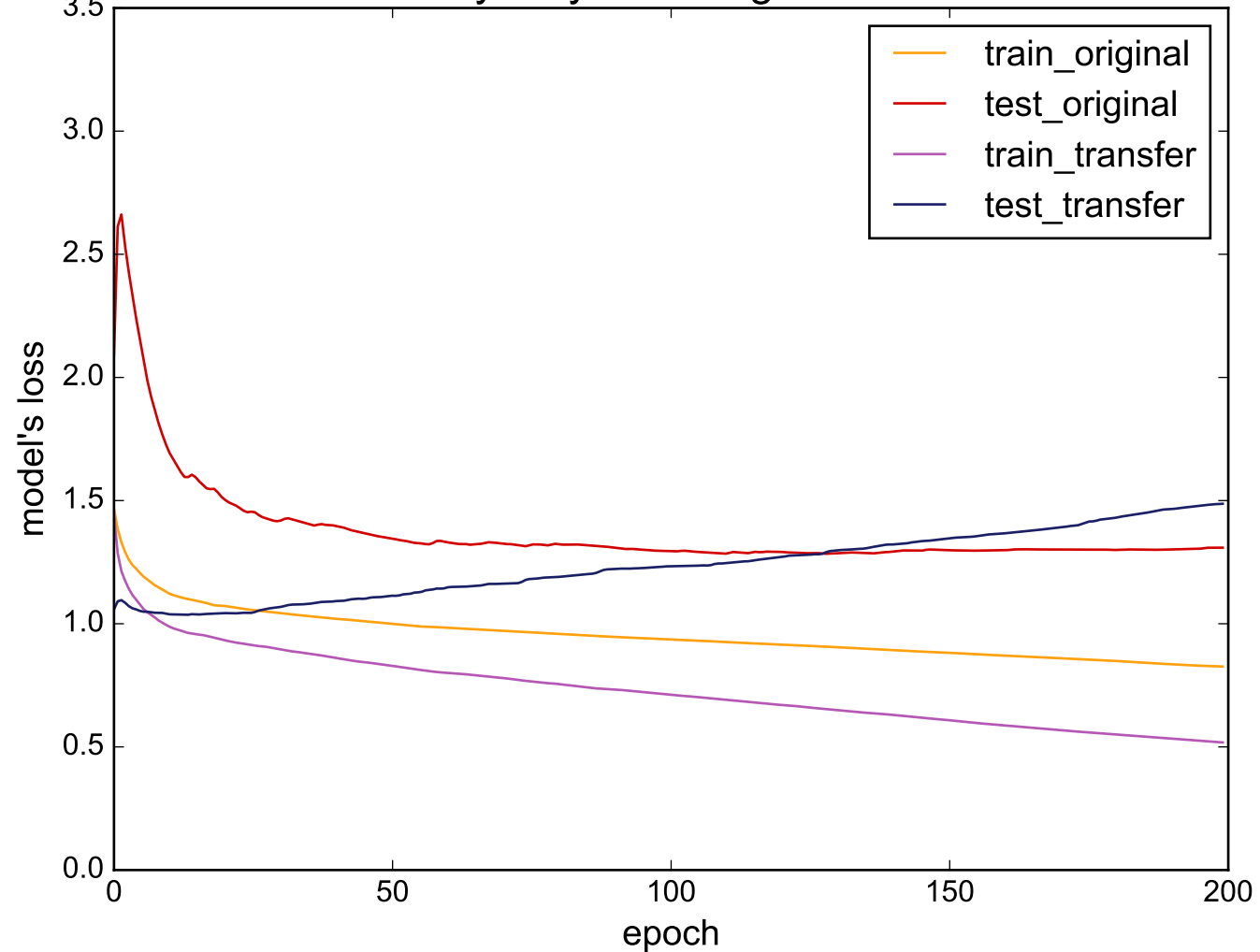
Source: WordsSynonyms - Target: MiddlePhalanxTW
