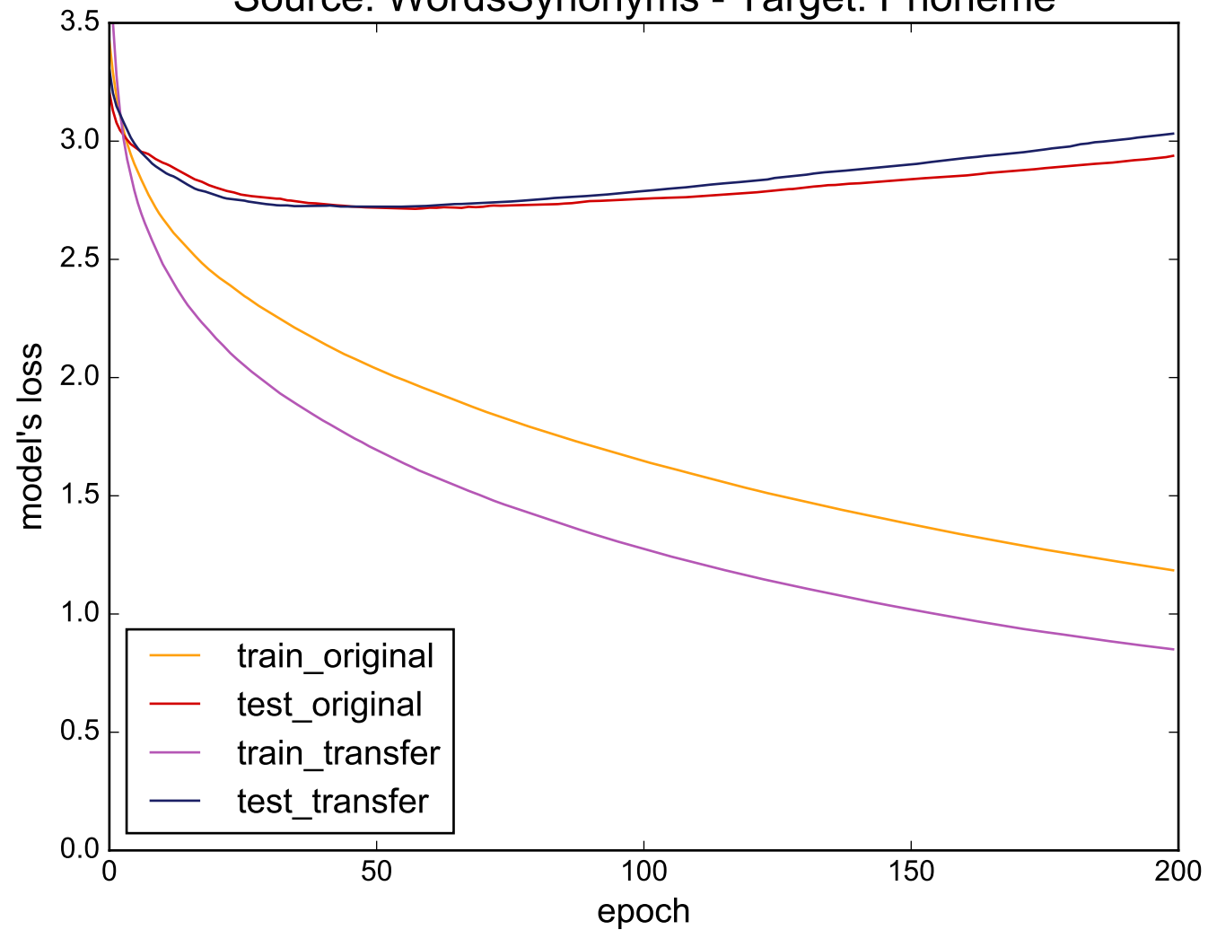
Source: WordsSynonyms - Target: Phoneme
