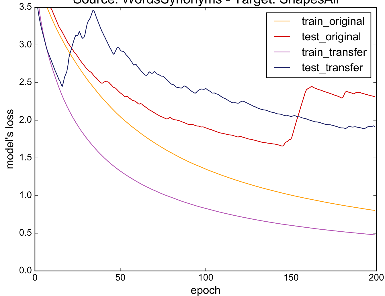
Source: WordsSynonyms - Target: ShapesAll
