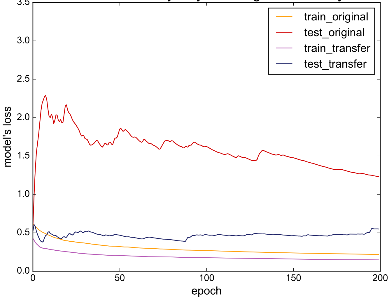
Source: WordsSynonyms - Target: Strawberry
