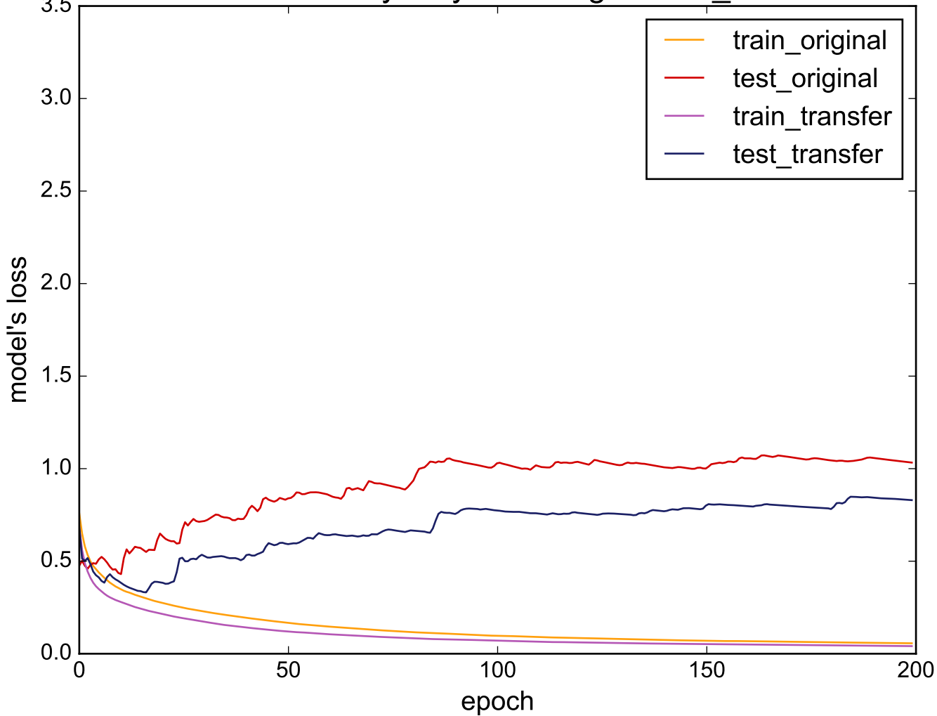
Source: WordsSynonyms - Target: Two_Patterns
