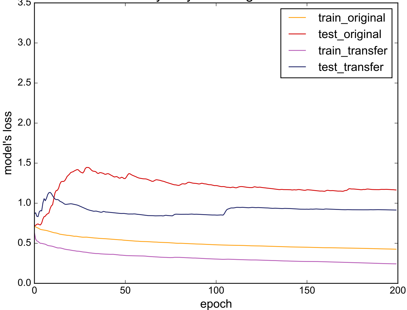
Source: WordsSynonyms - Target: WormsTwoClass
