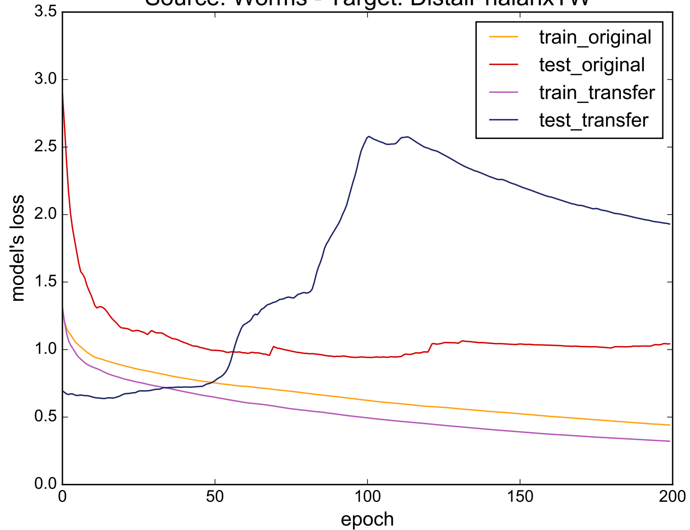
Source: Worms - Target: DistalPhalanxTW
