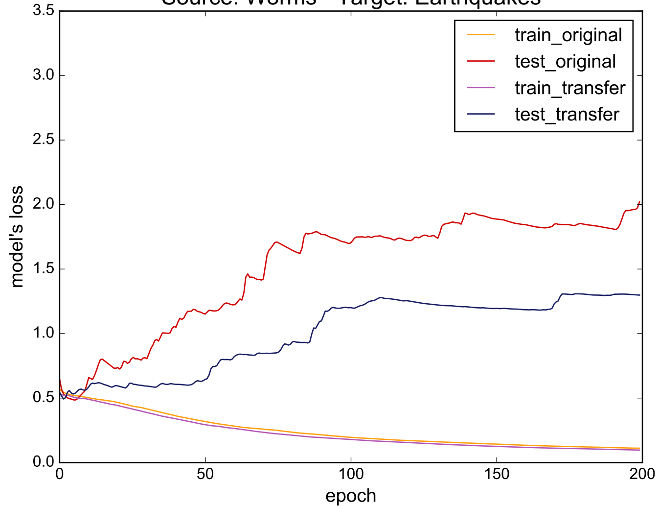
Source: Worms - Target: Earthquakes
