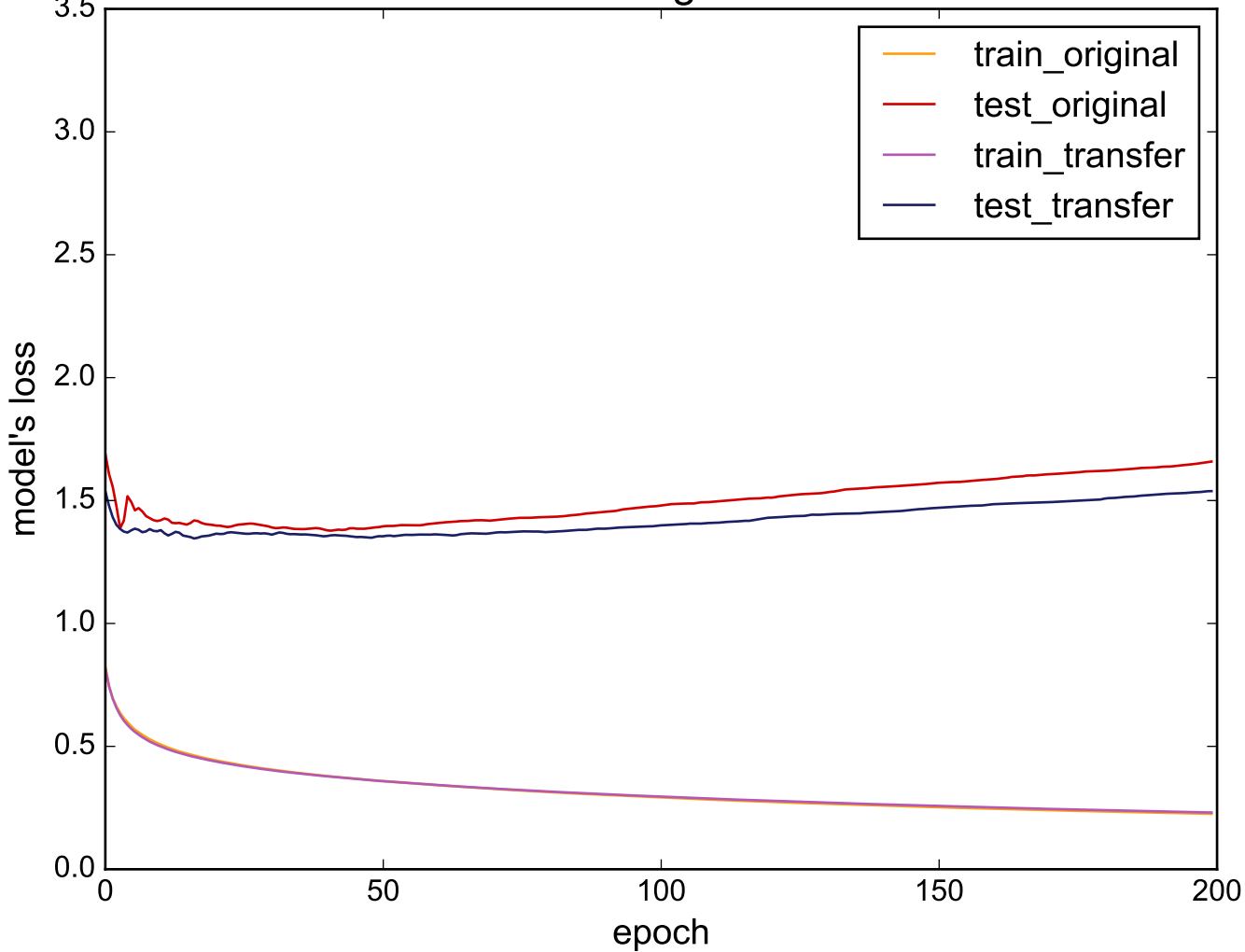
Source: Worms - Target: ElectricDevices
