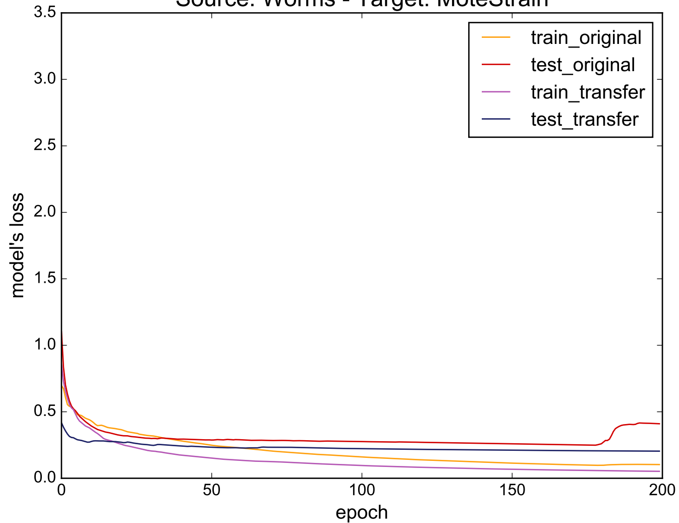
Source: Worms - Target: MoteStrain
