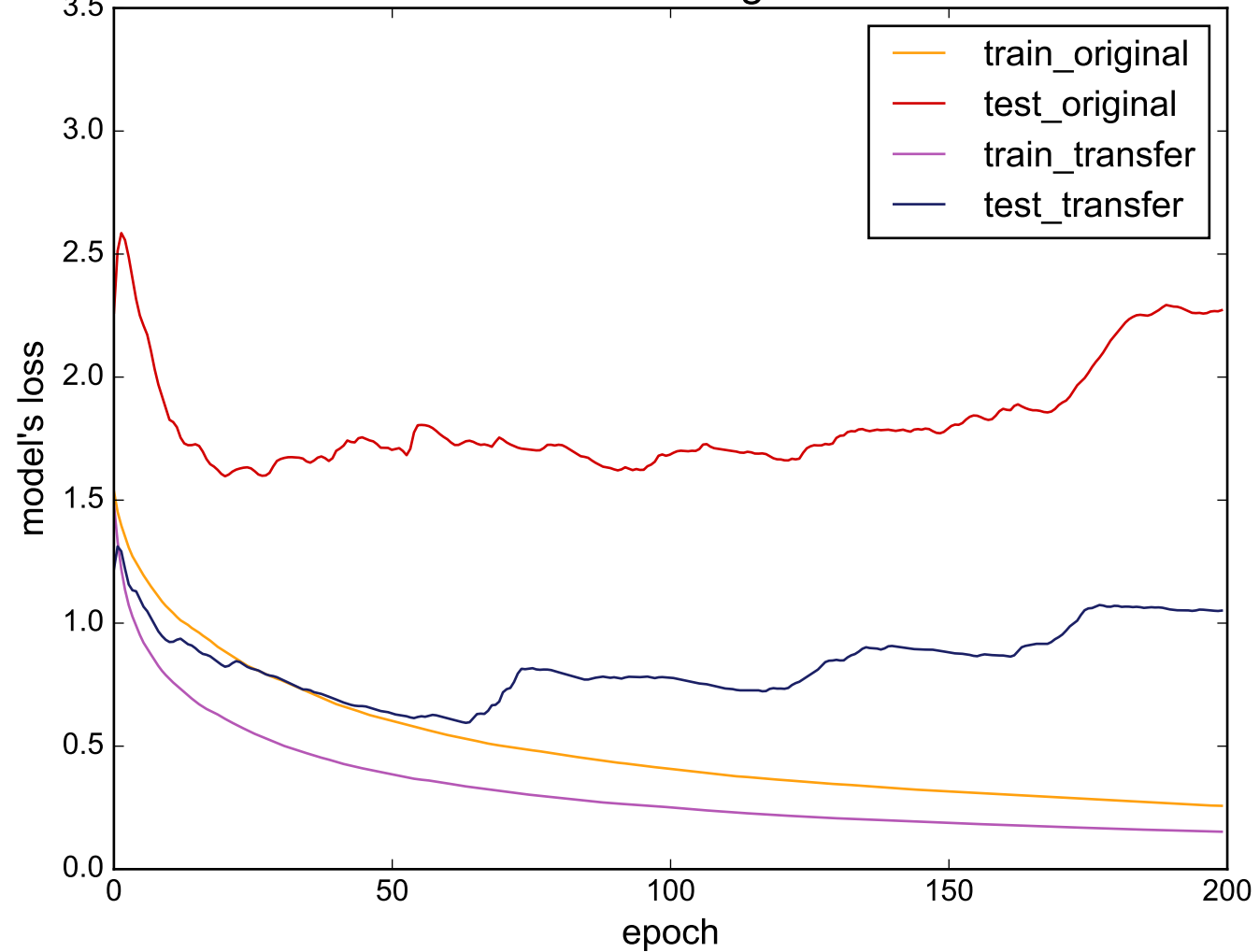
Source: Worms - Target: OSULeaf
