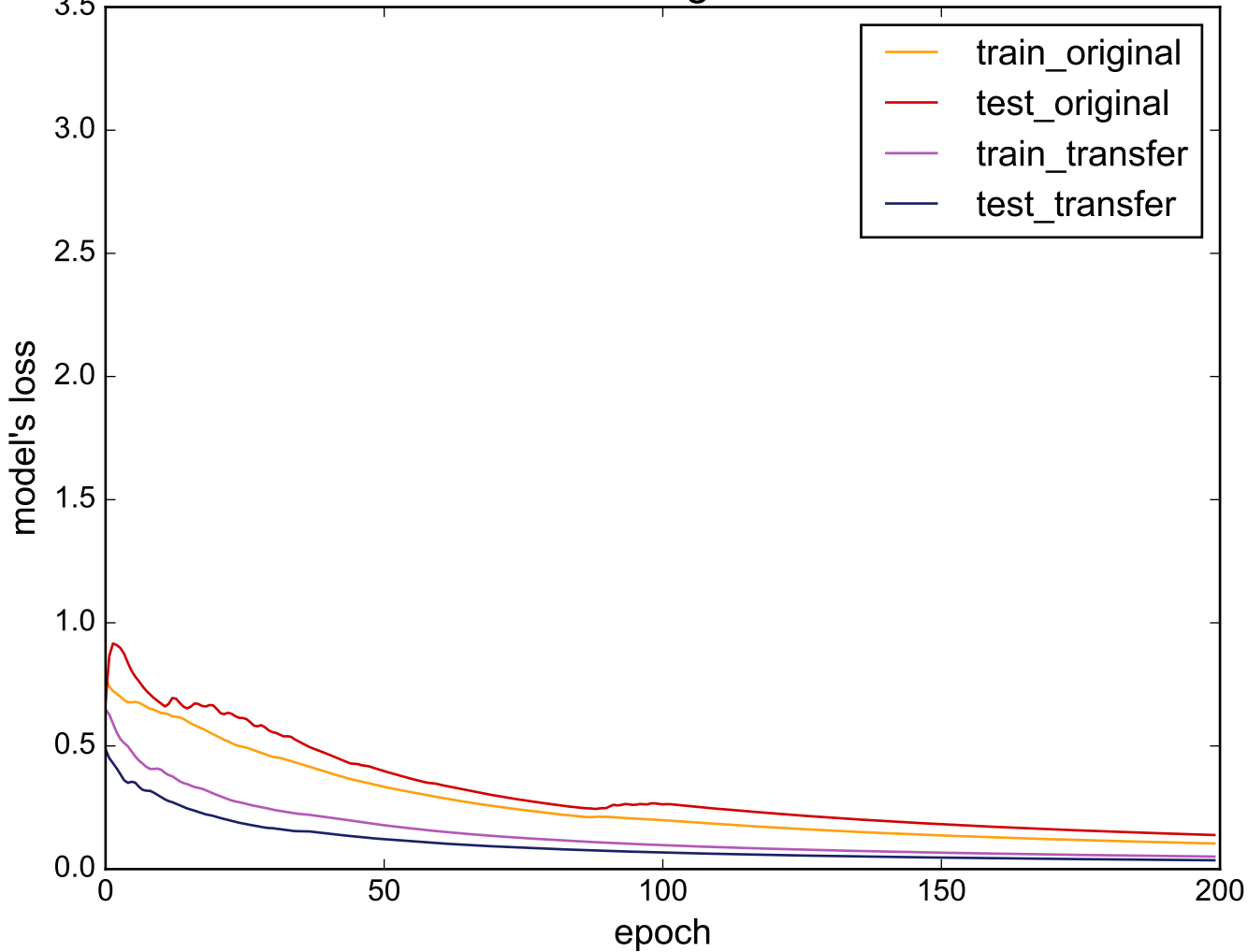
Source: Worms - Target: TwoLeadECG
