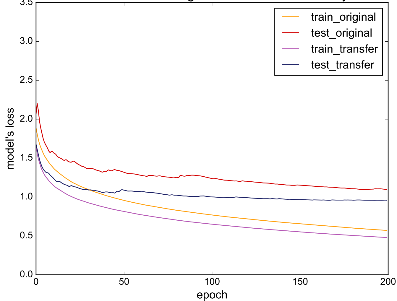
Source: Worms - Target: UWaveGestureLibraryAll
