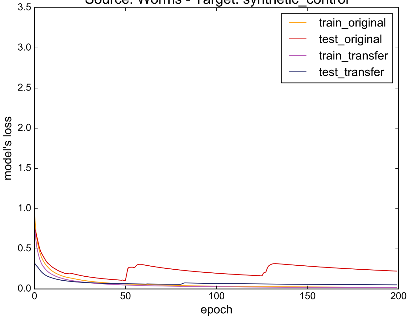
Source: Worms - Target: synthetic_control
