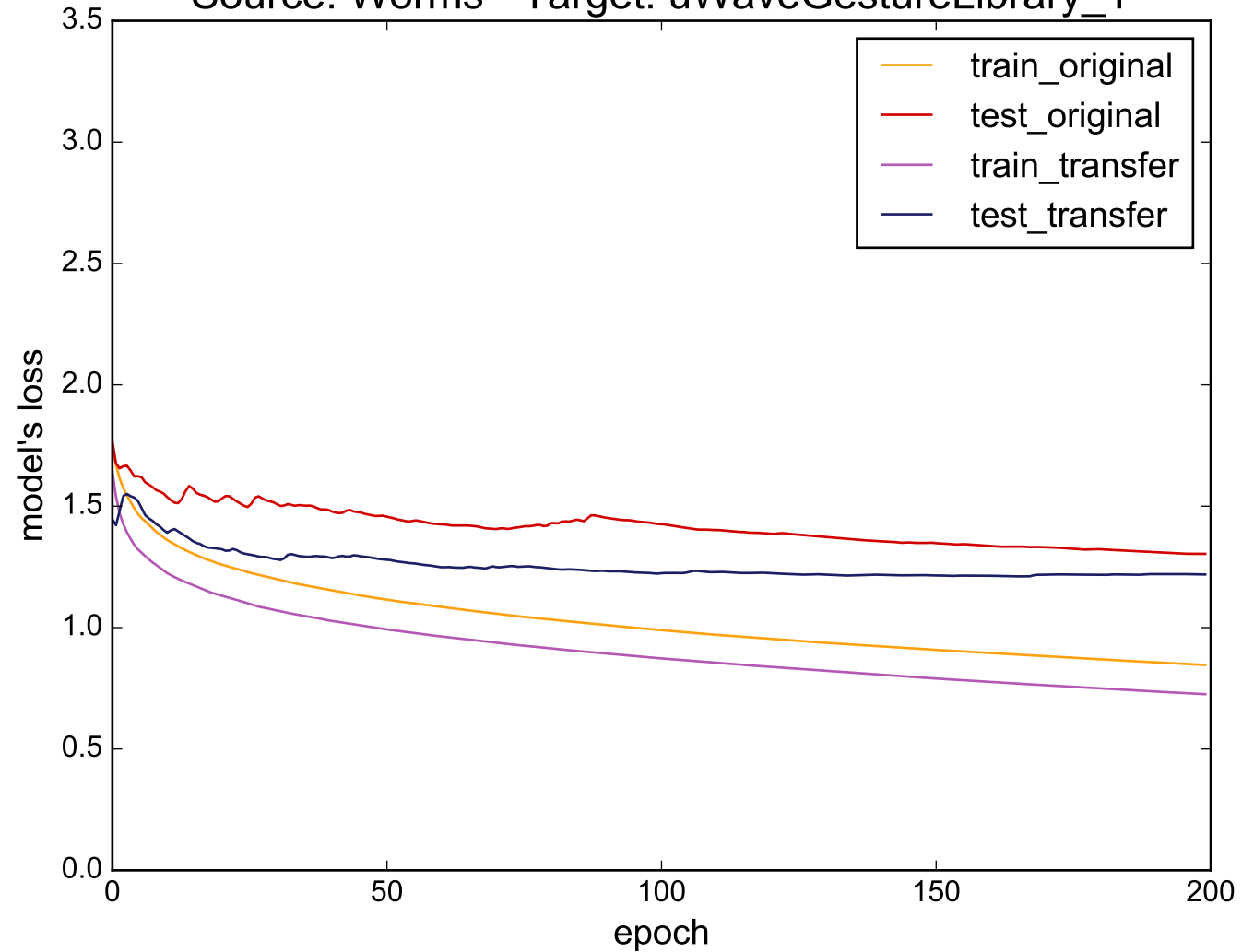
Source: Worms - Target: uWaveGestureLibrary_Y
