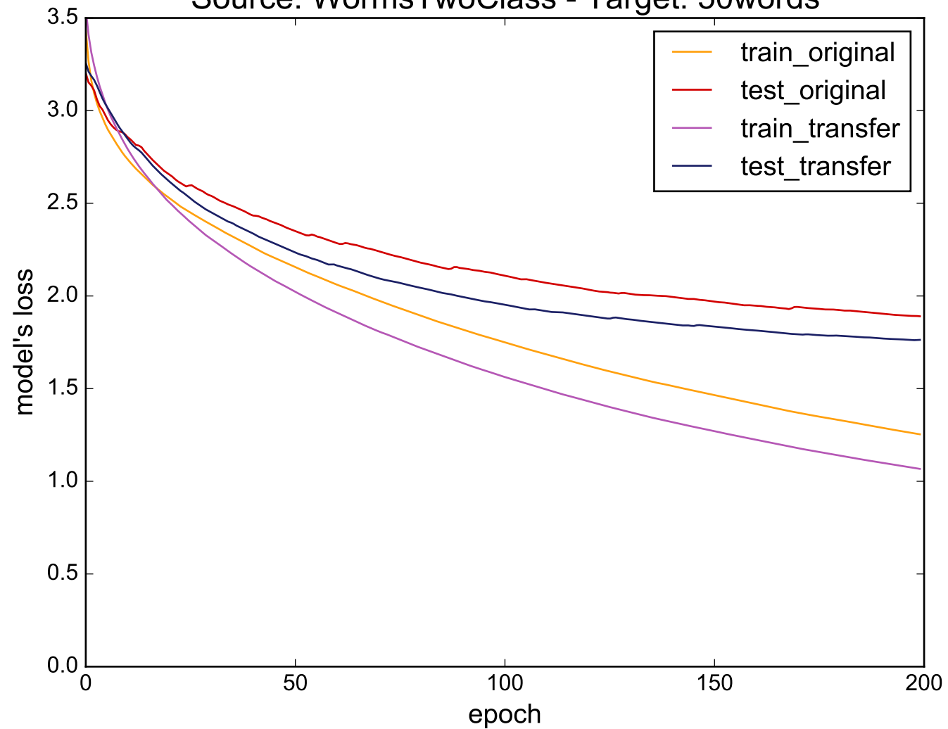
Source: WormsTwoClass - Target: 50words
