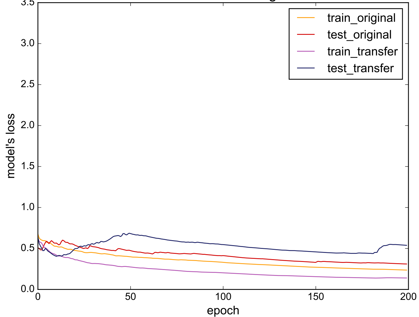
Source: WormsTwoClass - Target: BirdChicken
