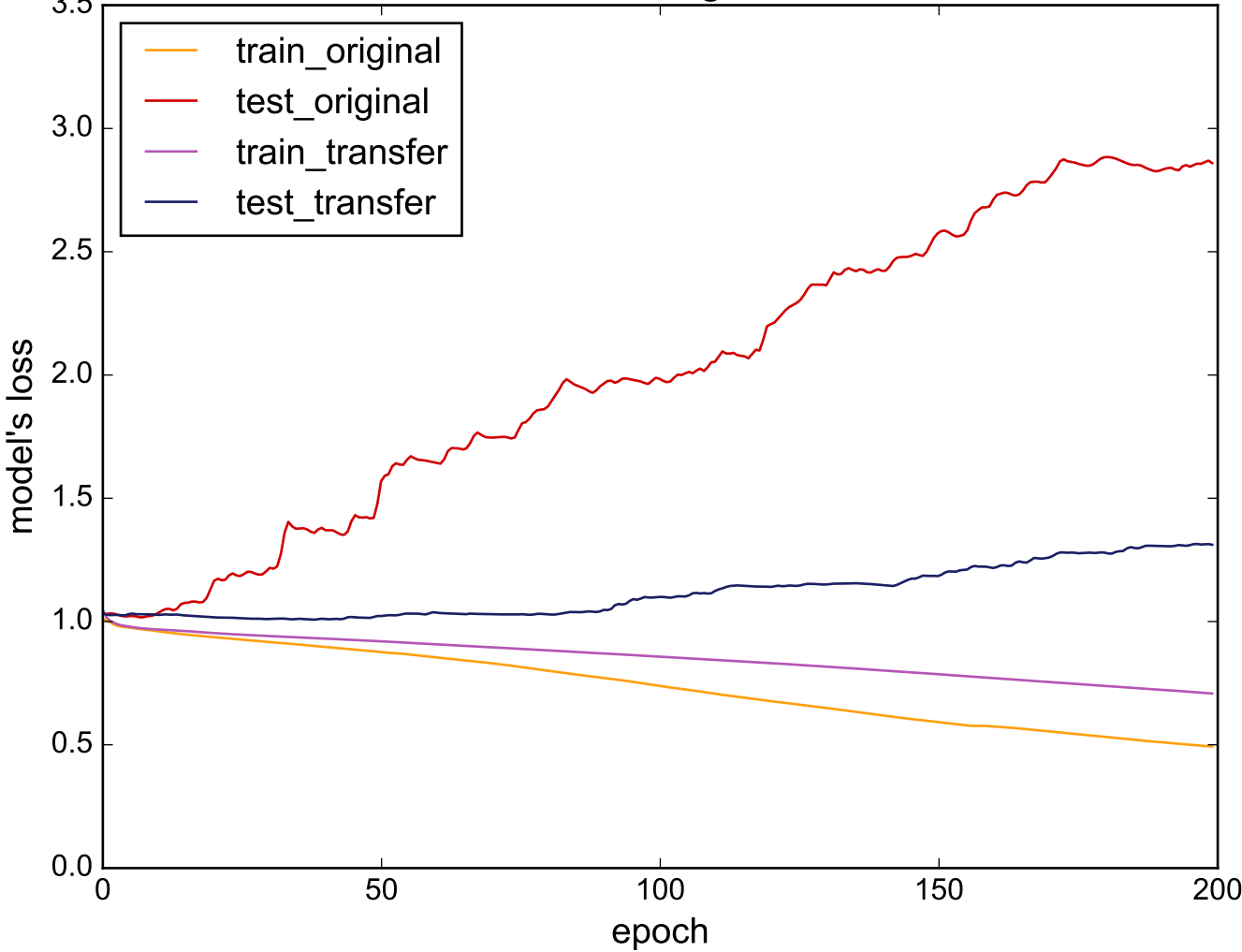
Source: WormsTwoClass - Target: ChlorineConcentration
