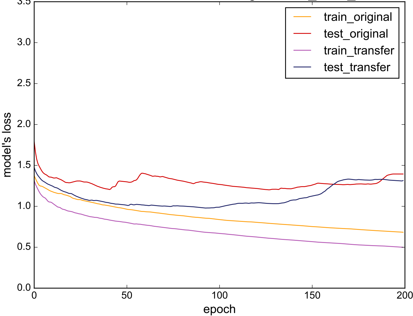
Source: WormsTwoClass - Target: CinC_ECG_torso
