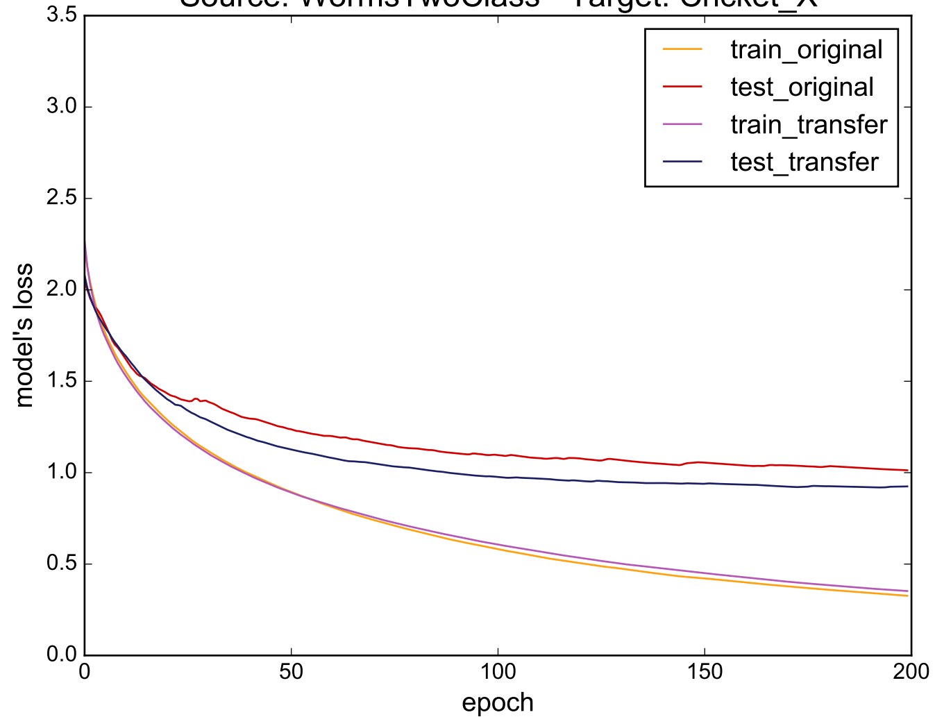
Source: WormsTwoClass - Target: Cricket_X
