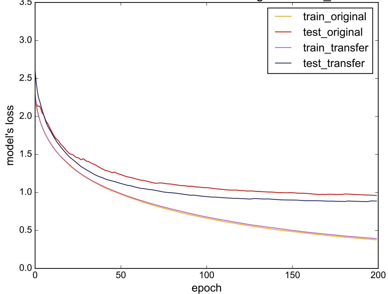
Source: WormsTwoClass - Target: Cricket_Z
