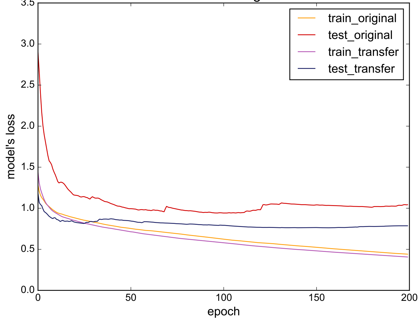
Source: WormsTwoClass - Target: DistalPhalanxTW
