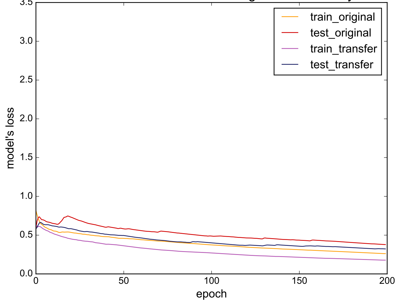
Source: WormsTwoClass - Target: ECGFiveDays
