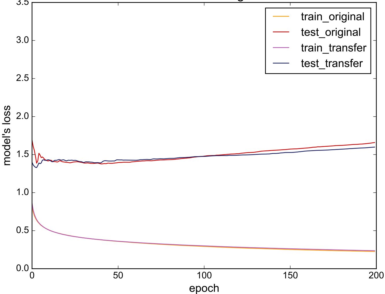
Source: WormsTwoClass - Target: ElectricDevices
