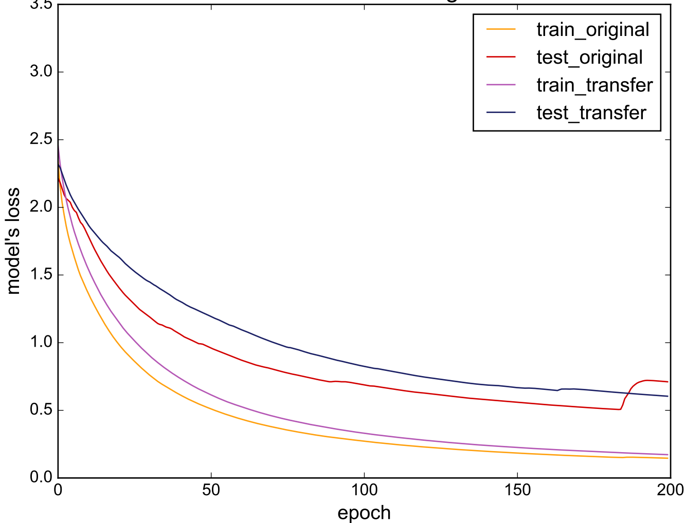
Source: WormsTwoClass - Target: FacesUCR
