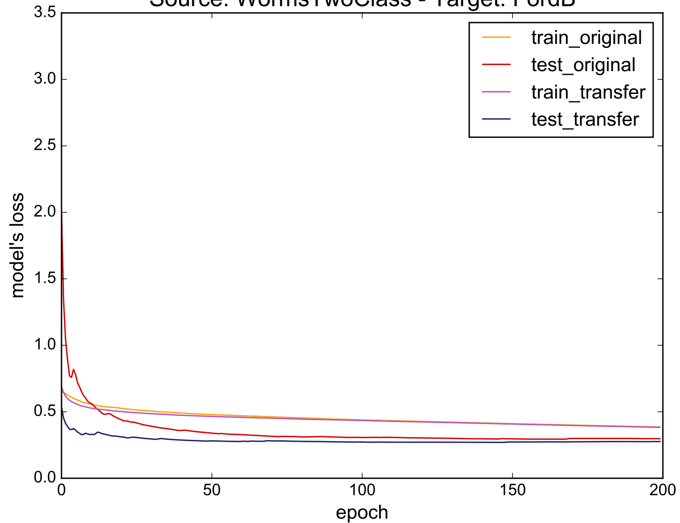
Source: WormsTwoClass - Target: FordB
