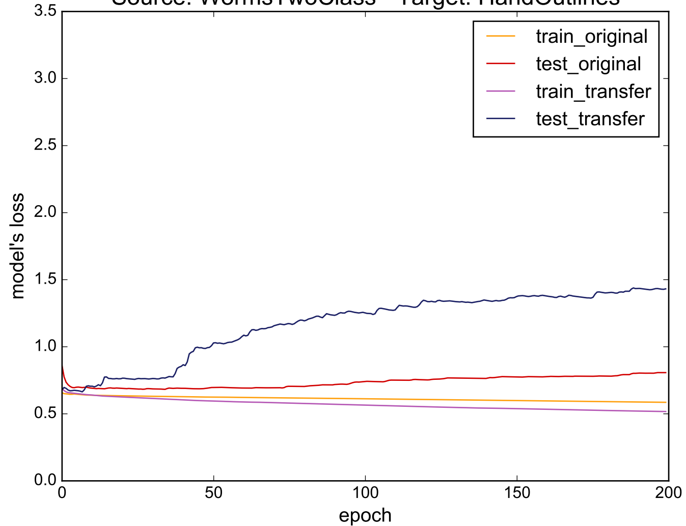
Source: WormsTwoClass - Target: HandOutlines
