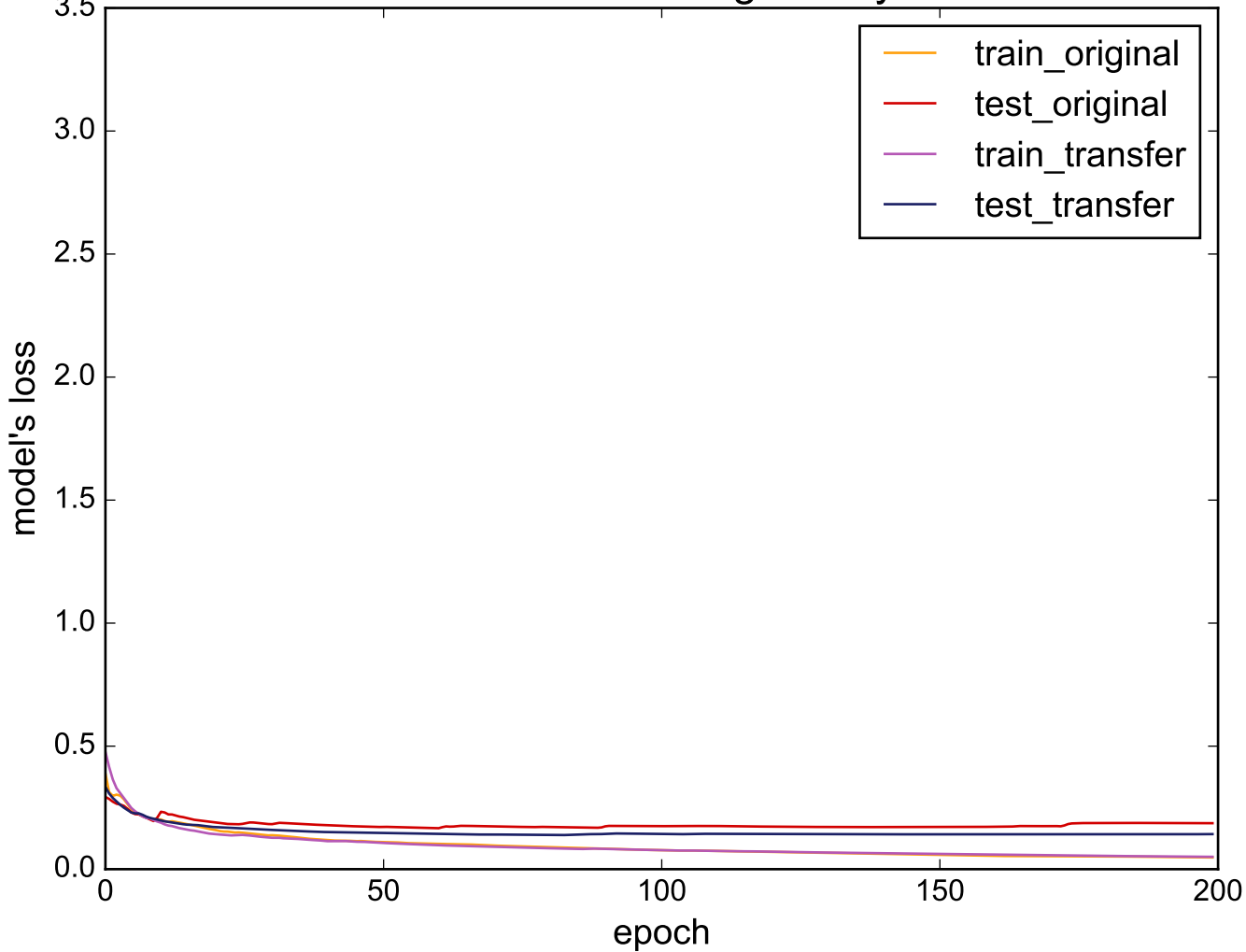
Source: WormsTwoClass - Target: ItalyPowerDemand
