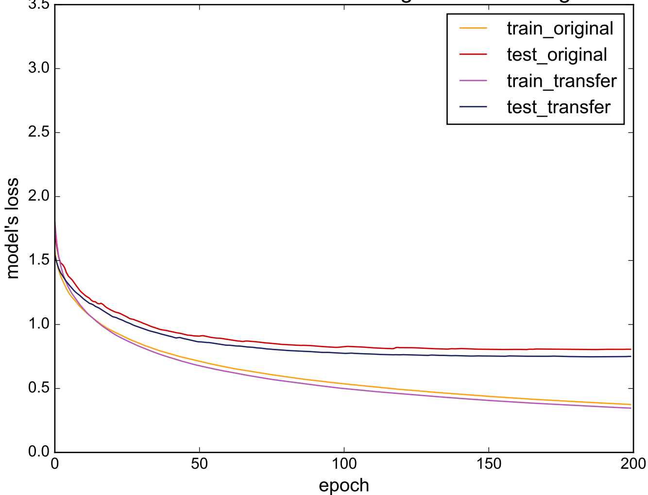
Source: WormsTwoClass - Target: MedicalImages
