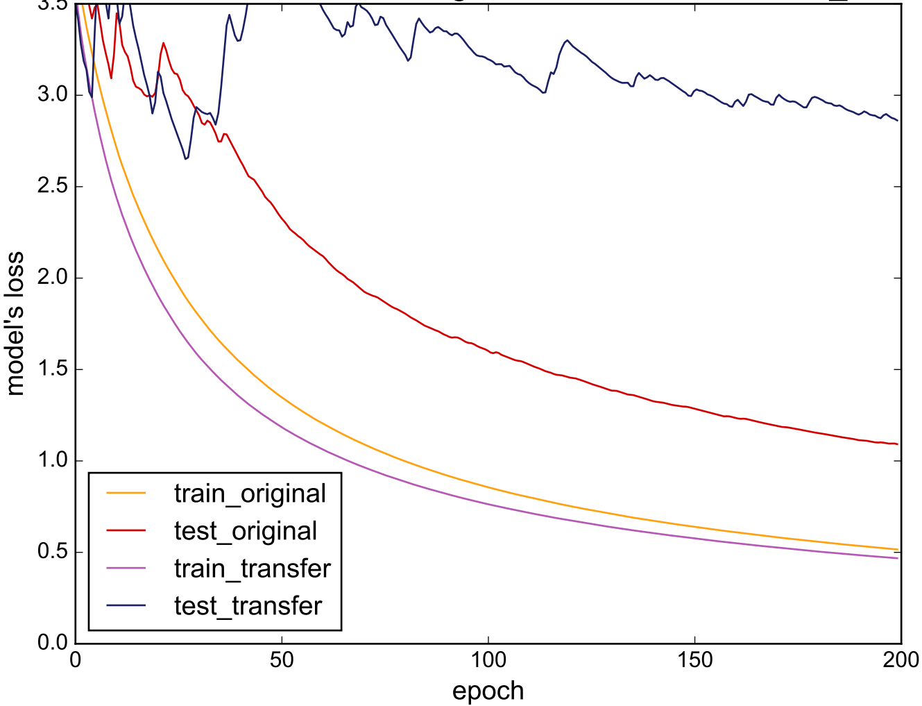
Source: WormsTwoClass - Target: NonInvasiveFatalECG_Thorax1
