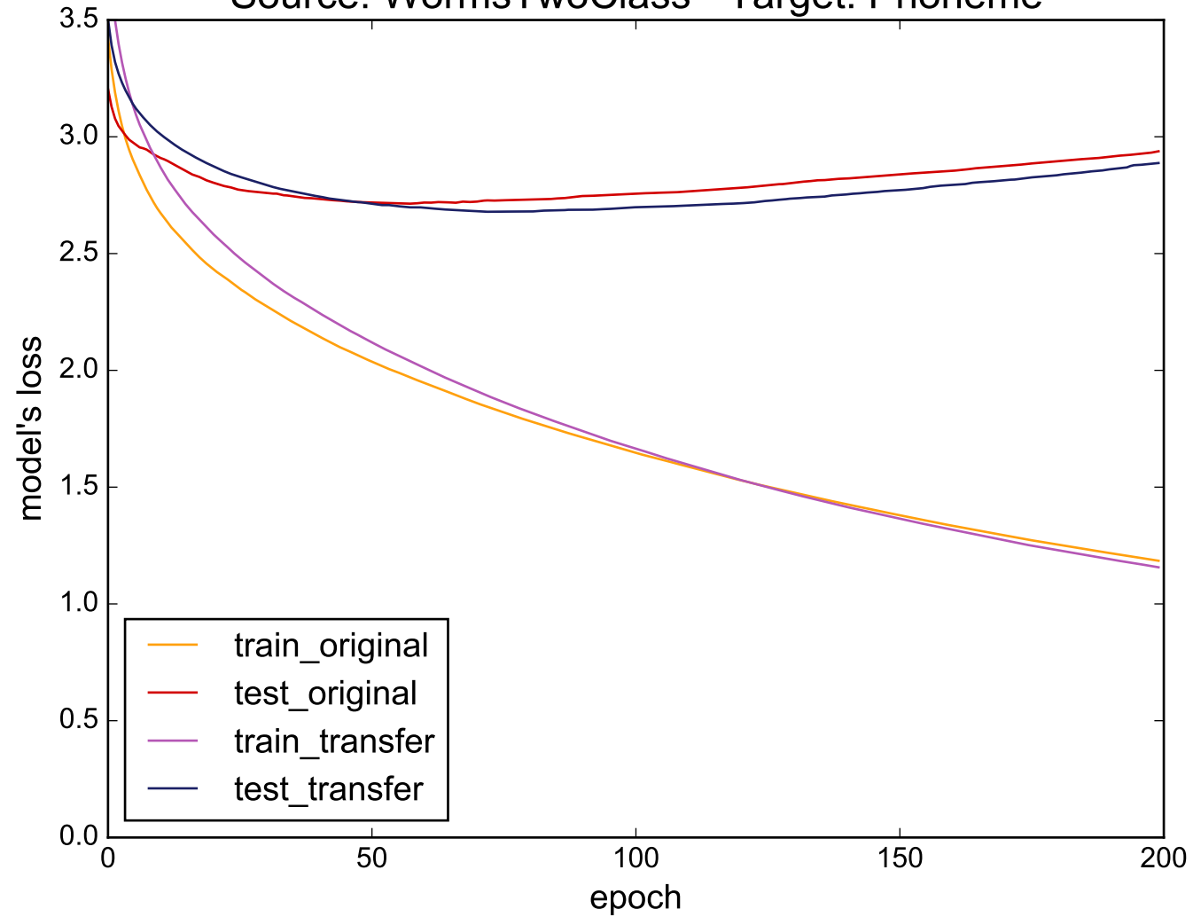
Source: WormsTwoClass - Target: Phoneme
