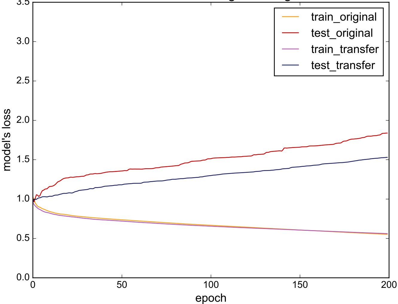
Source: WormsTwoClass - Target: RefrigerationDevices
