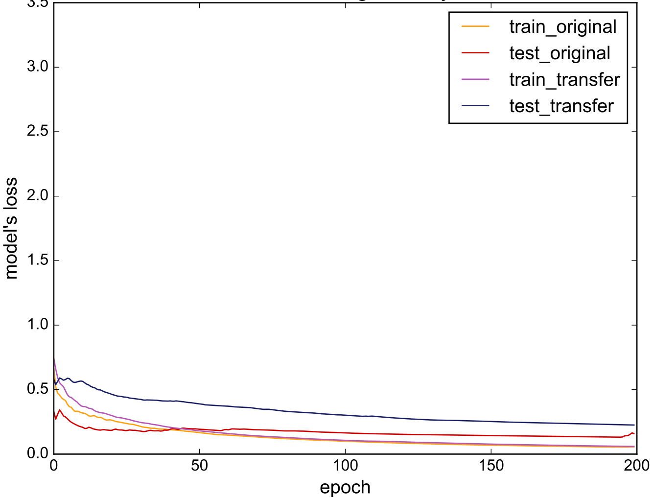
Source: WormsTwoClass - Target: SonyAIBORobotSurface
