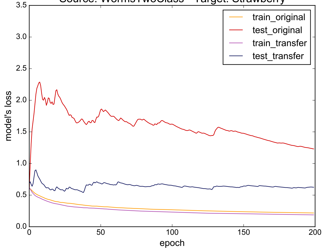
Source: WormsTwoClass - Target: Strawberry
