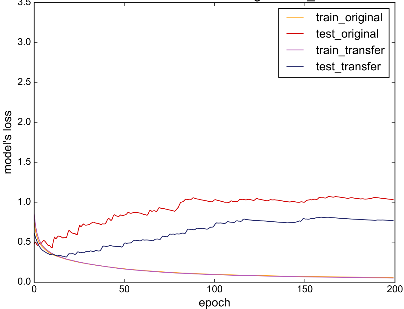
Source: WormsTwoClass - Target: Two_Patterns
