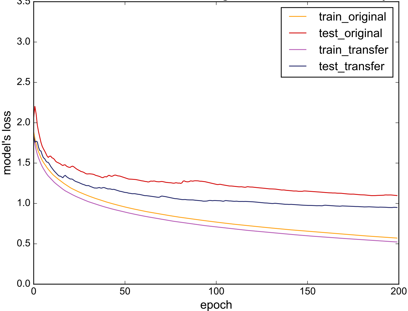
Source: WormsTwoClass - Target: UWaveGestureLibraryAll
