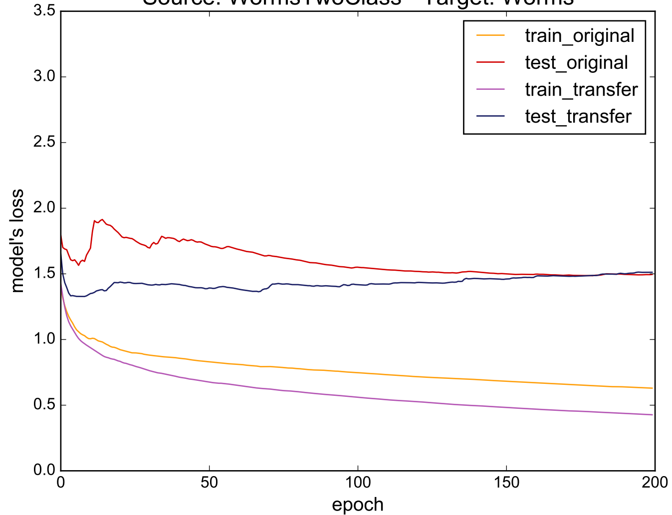
Source: WormsTwoClass - Target: Worms
