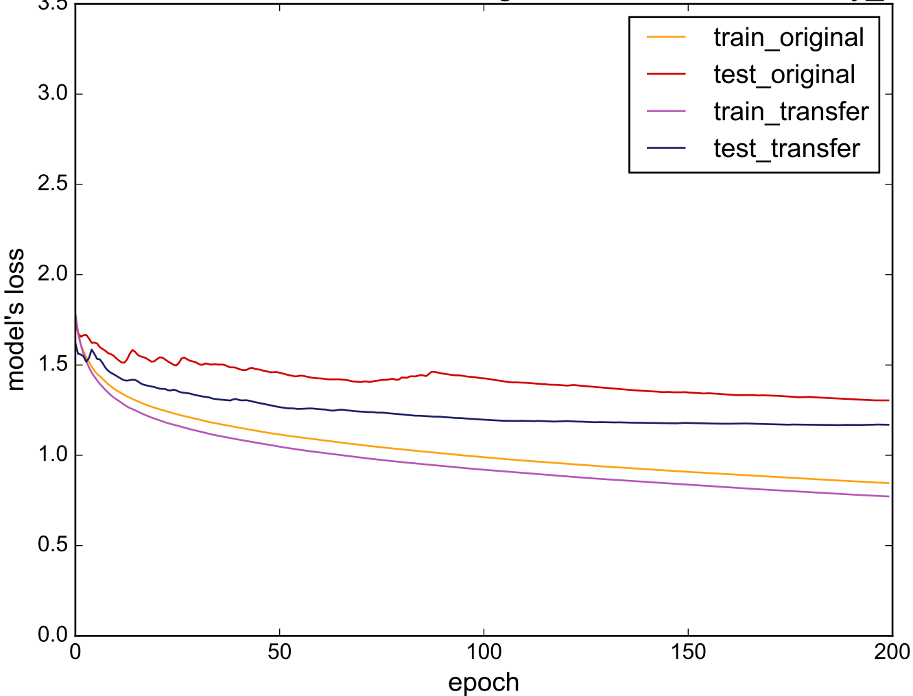
Source: WormsTwoClass - Target: uWaveGestureLibrary_Y
