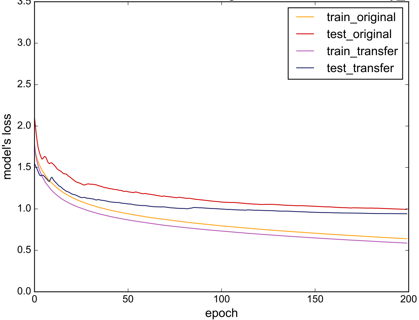
Source: WormsTwoClass - Target: uWaveGestureLibrary_Z
