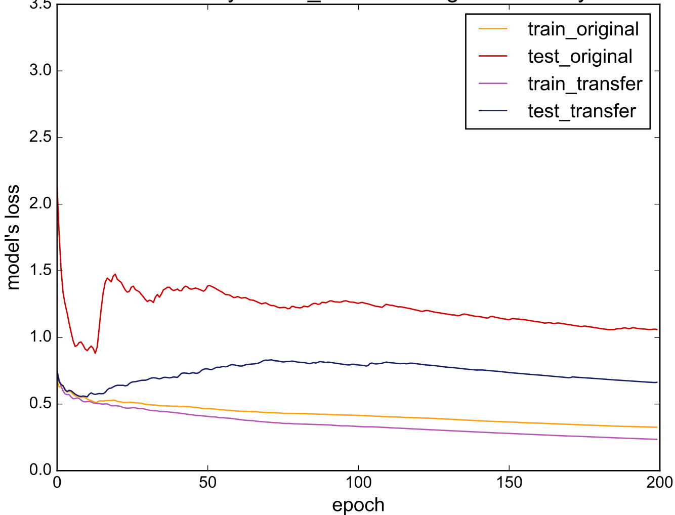
Source: synthetic_control - Target: BeetleFly
