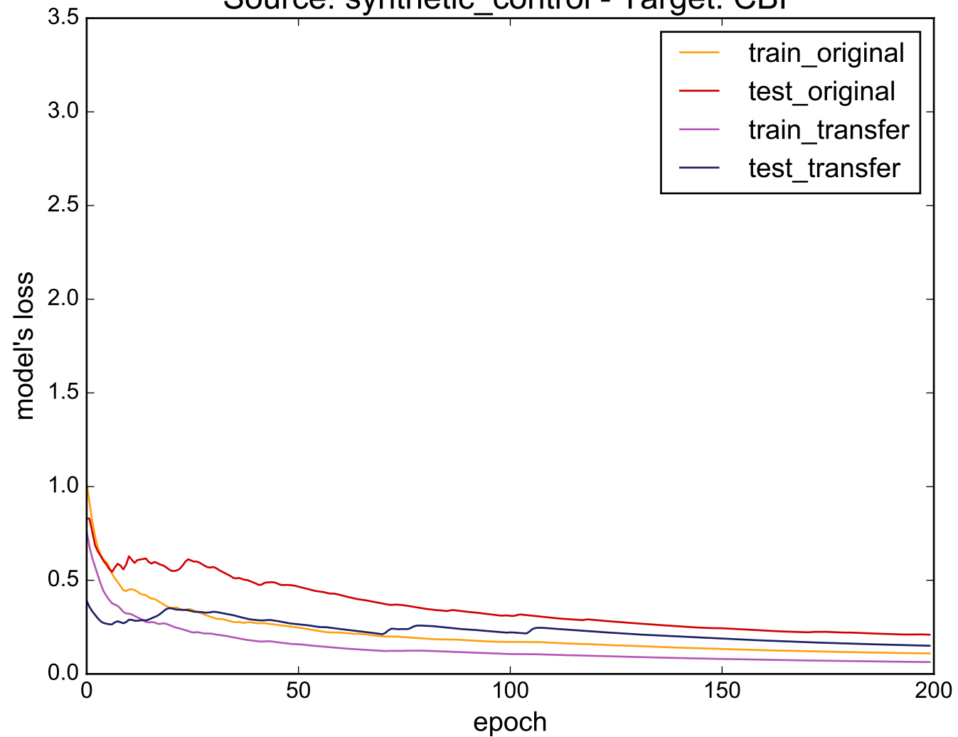
Source: synthetic_control - Target: CBF
