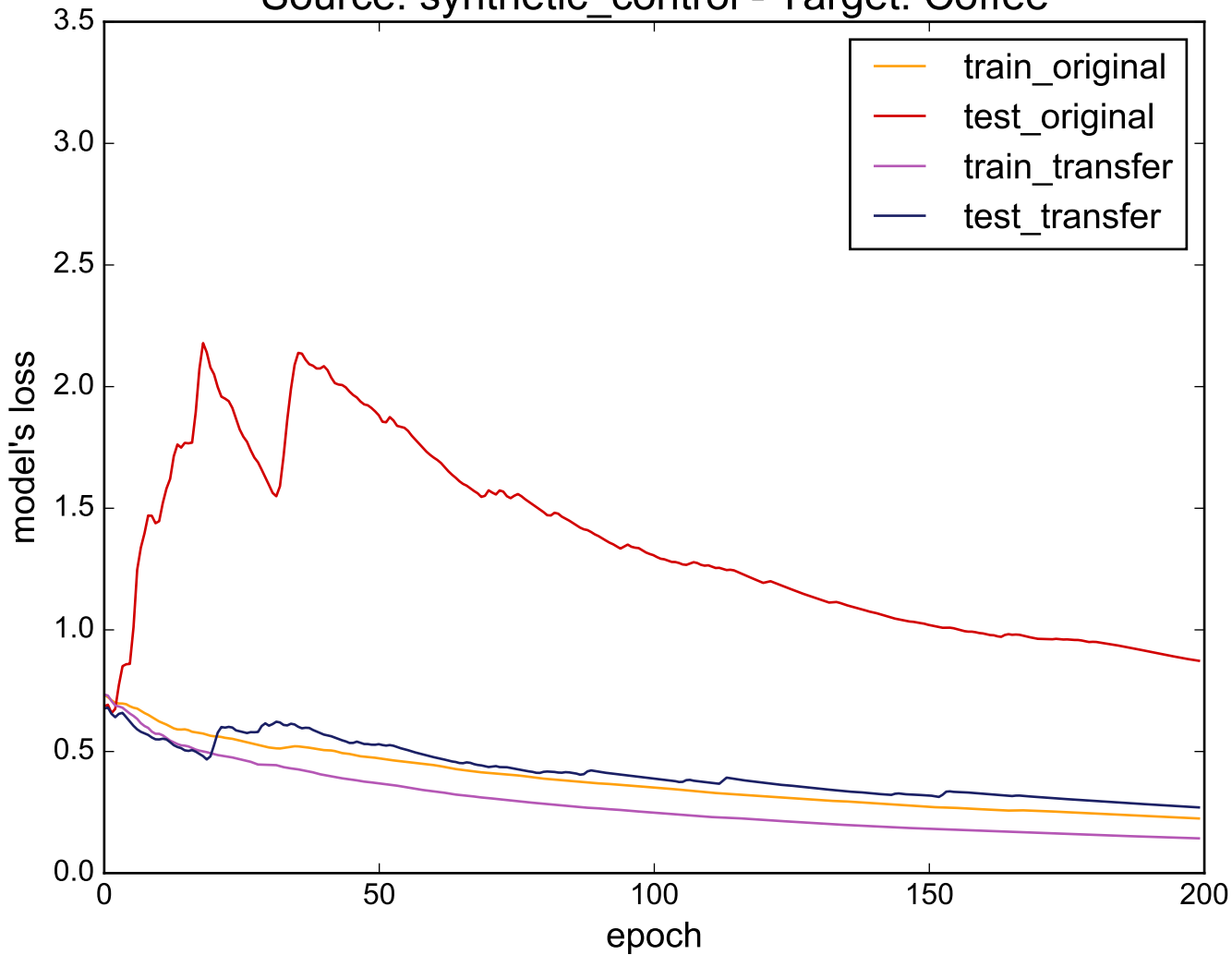
Source: synthetic_control - Target: Coffee
