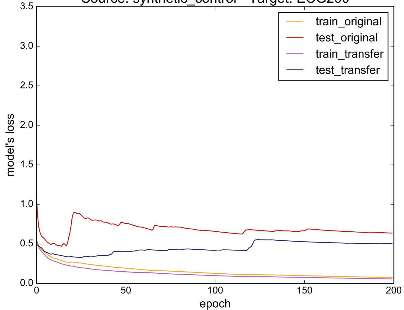
Source: synthetic_control - Target: ECG200
